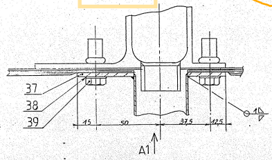
DETAIL 4
