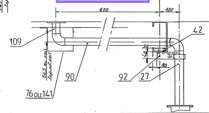
CÔUPE ZZ SECTION .
