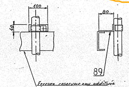
DETAIL 5
