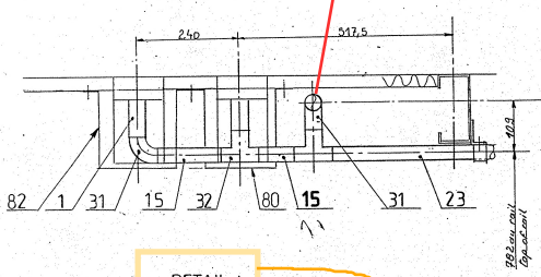
DETAIL 4
