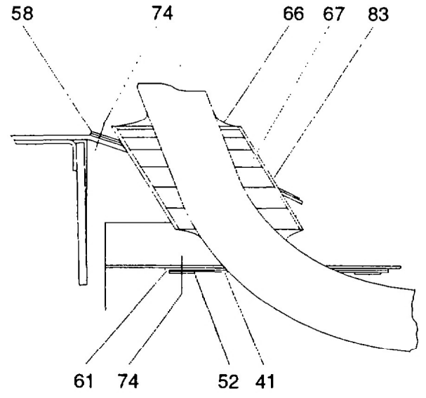
SECTION L
