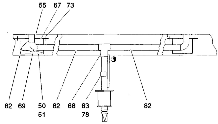
SECTION J
