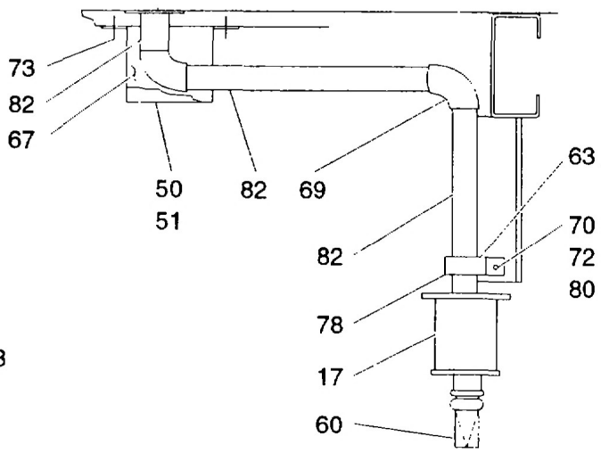
SECTION E
