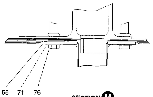
SECTION M
